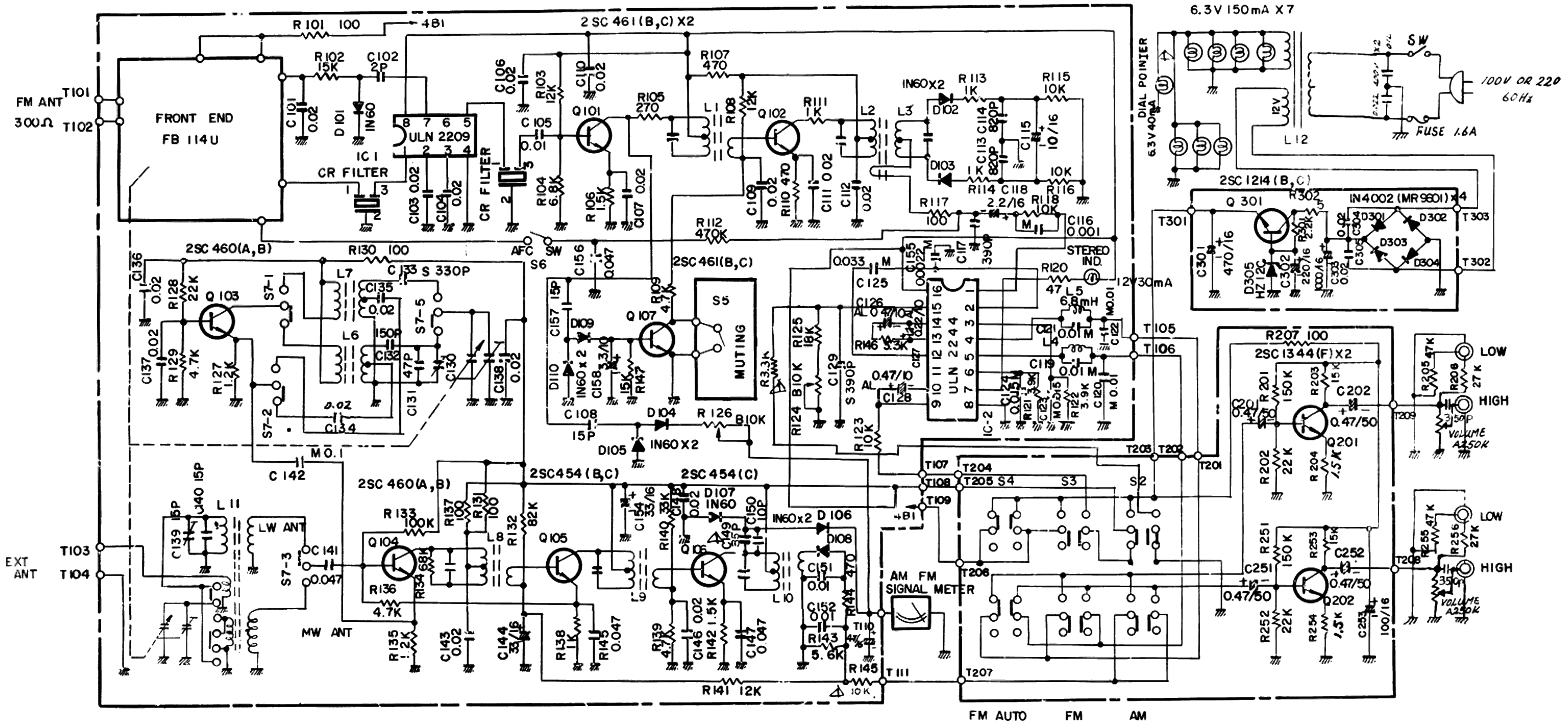
SCHMATIC DIAGRAM FOR MODEL ID-303
